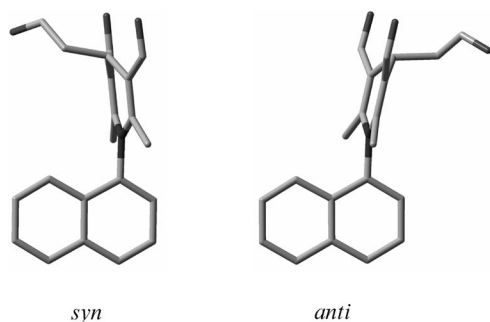
Figure 1. DFT calculated syn and anti conformers of 7g . Hydrogen atoms and OEt groups are omitted for clarity.
