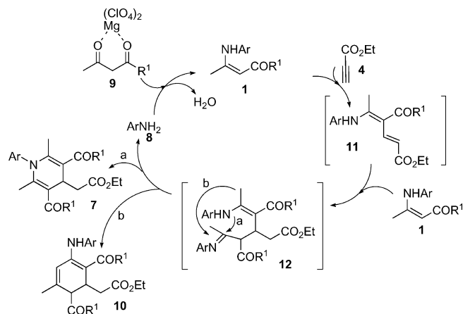
Scheme 3. A plausible mechanism proposed for the reaction.
